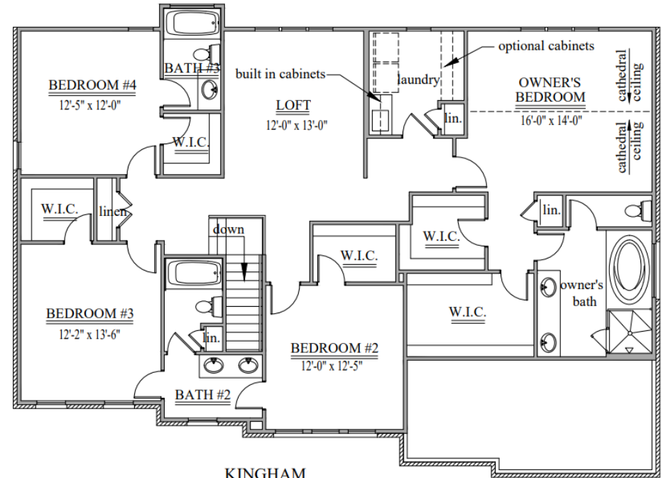
KINGHAM SECOND FLOOR PLAN 1834 s.f.
