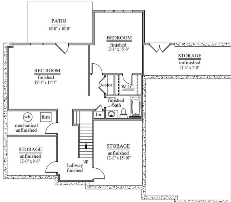
KINGHAM BASEMENT FLOOR PLAN 865 s.f. finished
