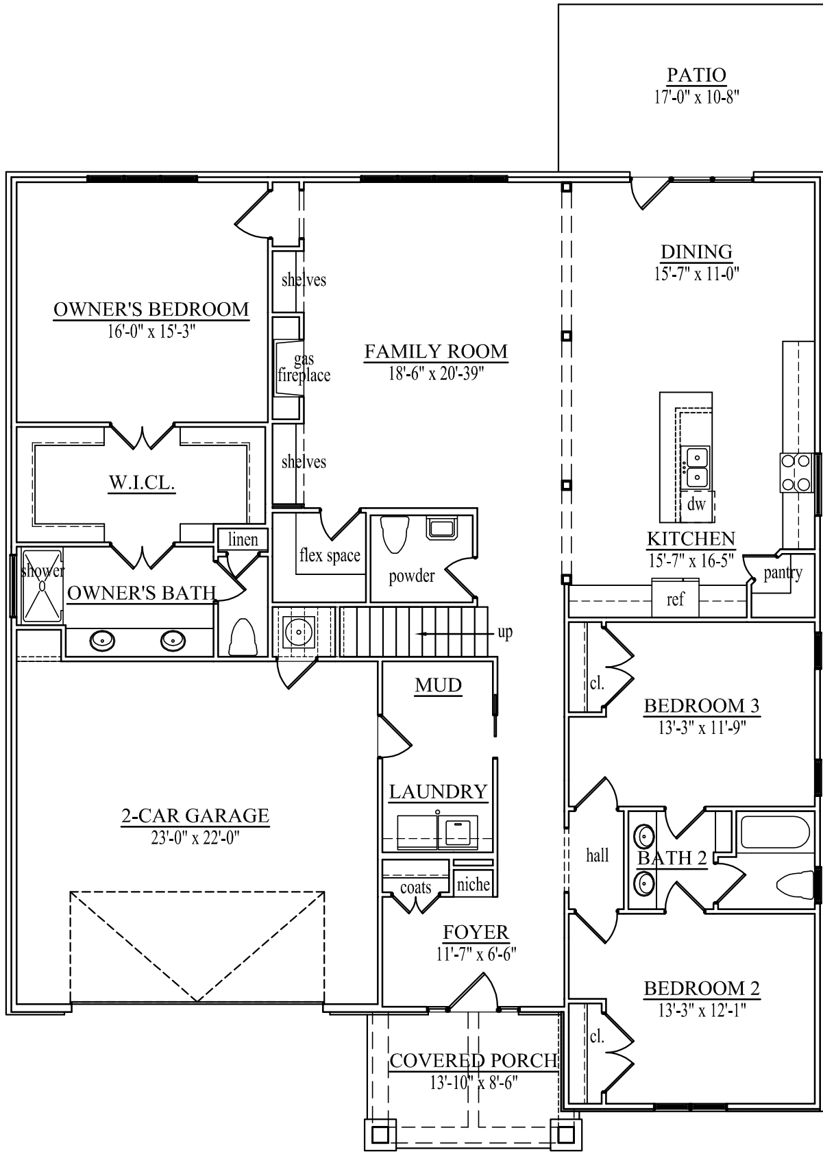
ASHEVILLE FIRST FLOOR PLAN 2,318 s.f.
