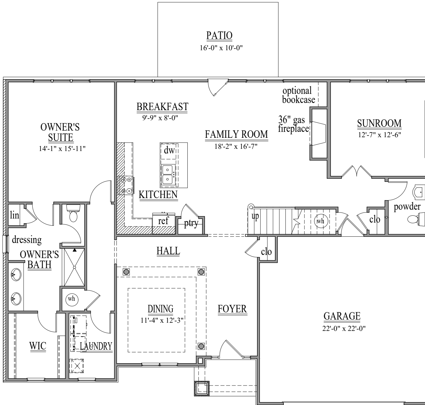
AFTON FLOOR PLAN 1795 s.f.
