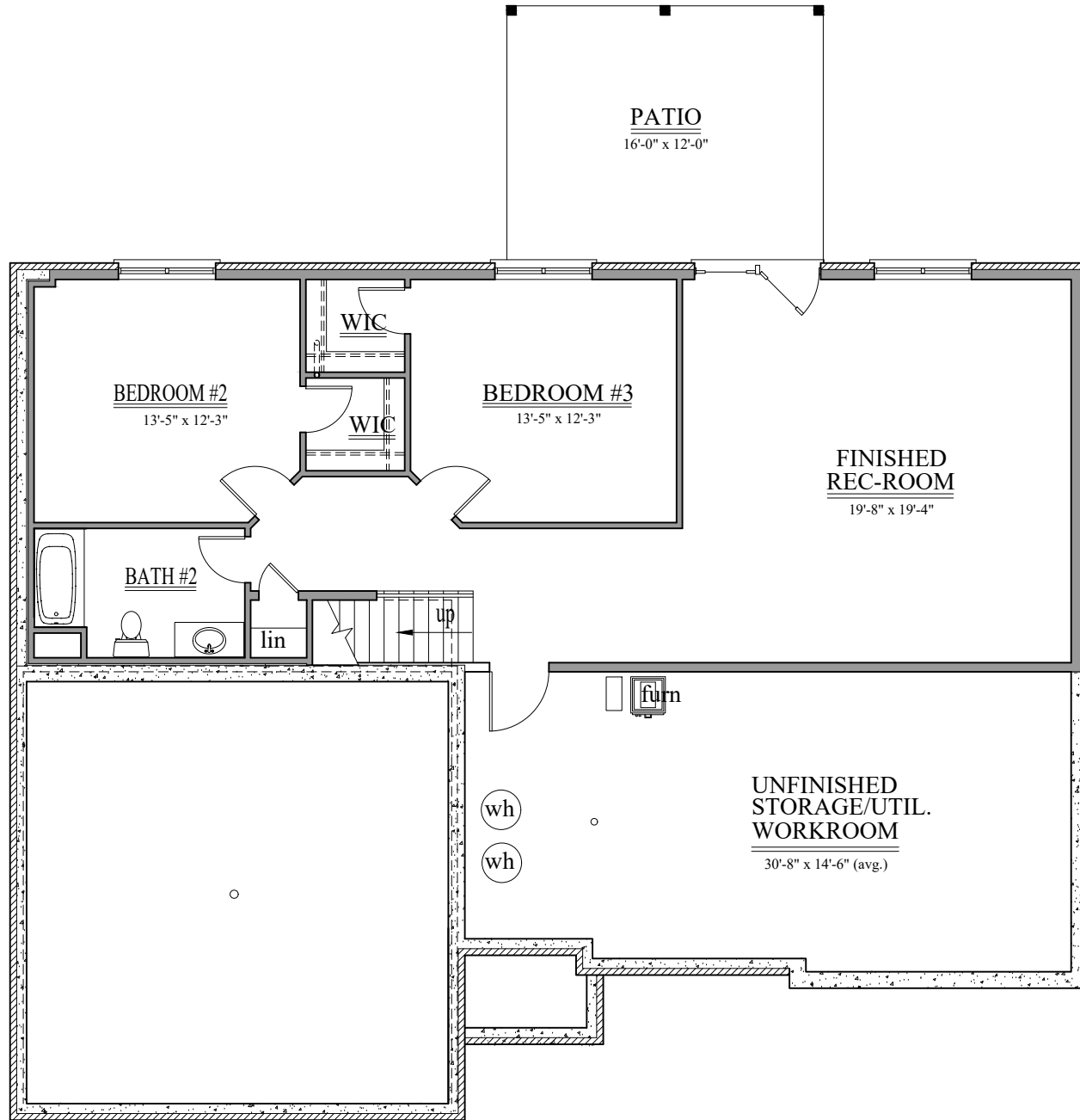
"KENTMERE" BASEMENT PLAN 1138 s.f. finished
