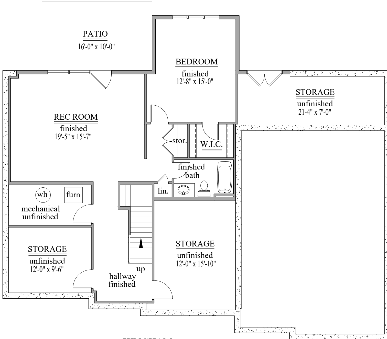
KINGHAM BASEMENT FLOOR PLAN 865 s.f. finished
